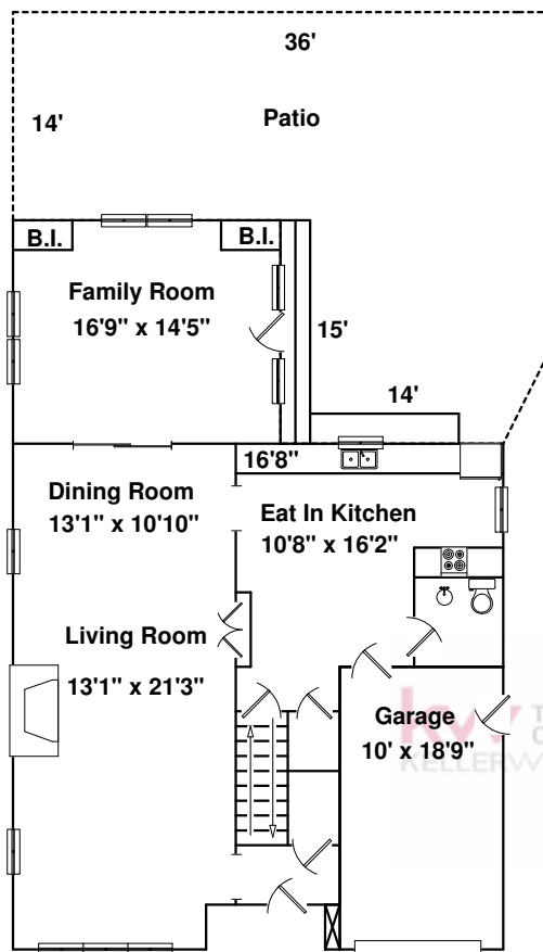
Main level
